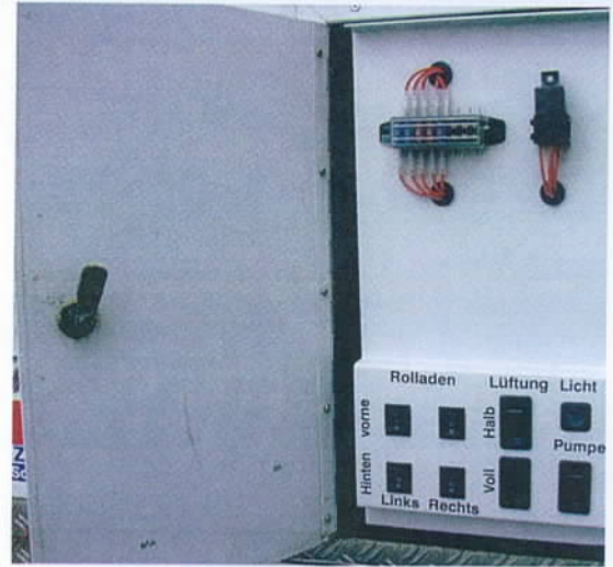
Electr. Control of the shutters, waterpump, air-ventilation-system and the lights
