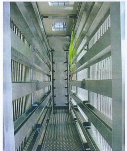
Middle corridor with non slip checker plate, skylights, patented revolving drinking system, water supply and air ventilation for every single crate
