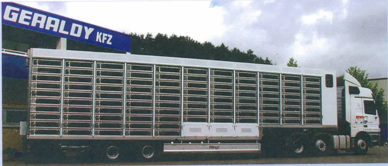
Articulated trailers for app. 6.000 pigeons
